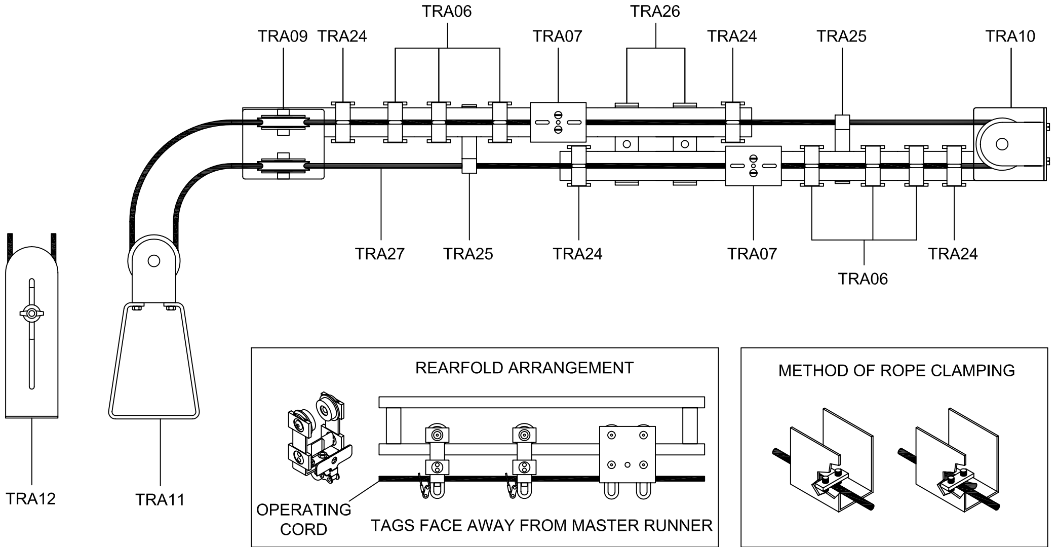
CORDING DIAGRAM 01 STANDARD CENTRE OVERLAP TRACK (VIEWED FROM UNDERSIDE)
