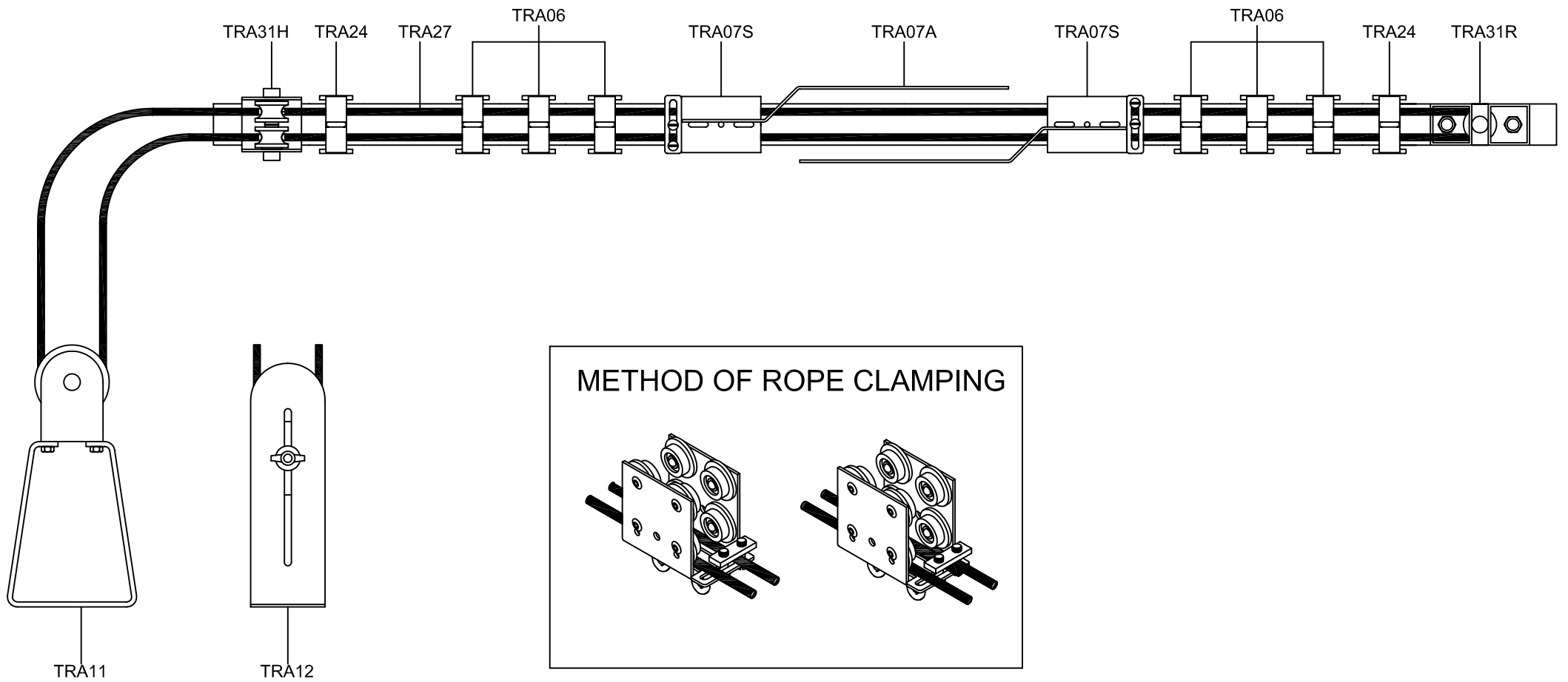
CORDING DIAGRAM 06 SINGLE TRACK WITH CENTRE OVERLAPPING ARMS VIEWED FROM UNDERSIDE
