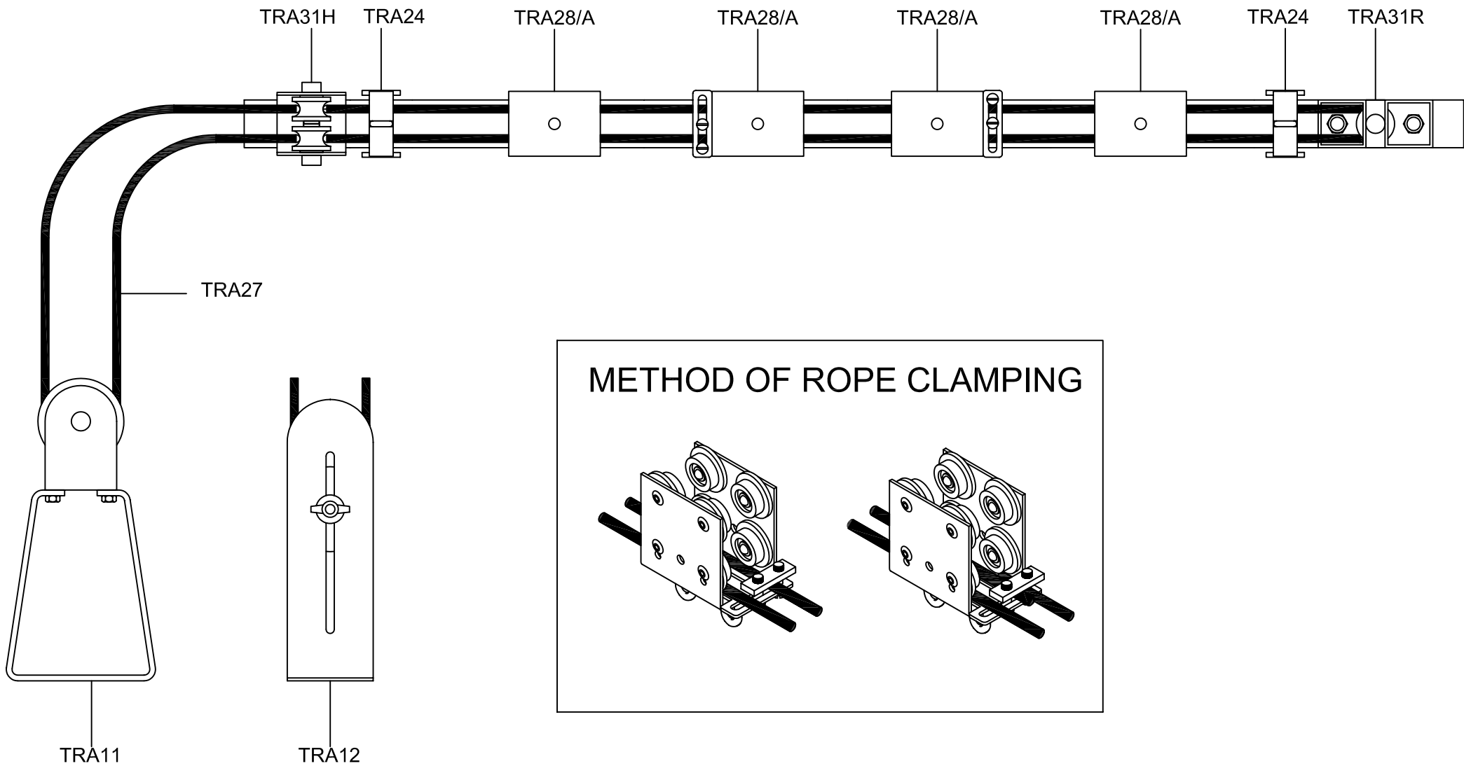
CORDING DIAGRAM 07 SINGLE TRACK WITH CENTRE BUTTING SCENERY VIEWED FROM UNDERSIDE
