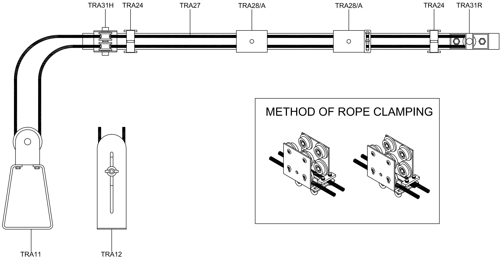
CORDING DIAGRAM 08 SINGLE TRACK WIPE FOR SCENERY VIEWED FROM UNDERSIDE
