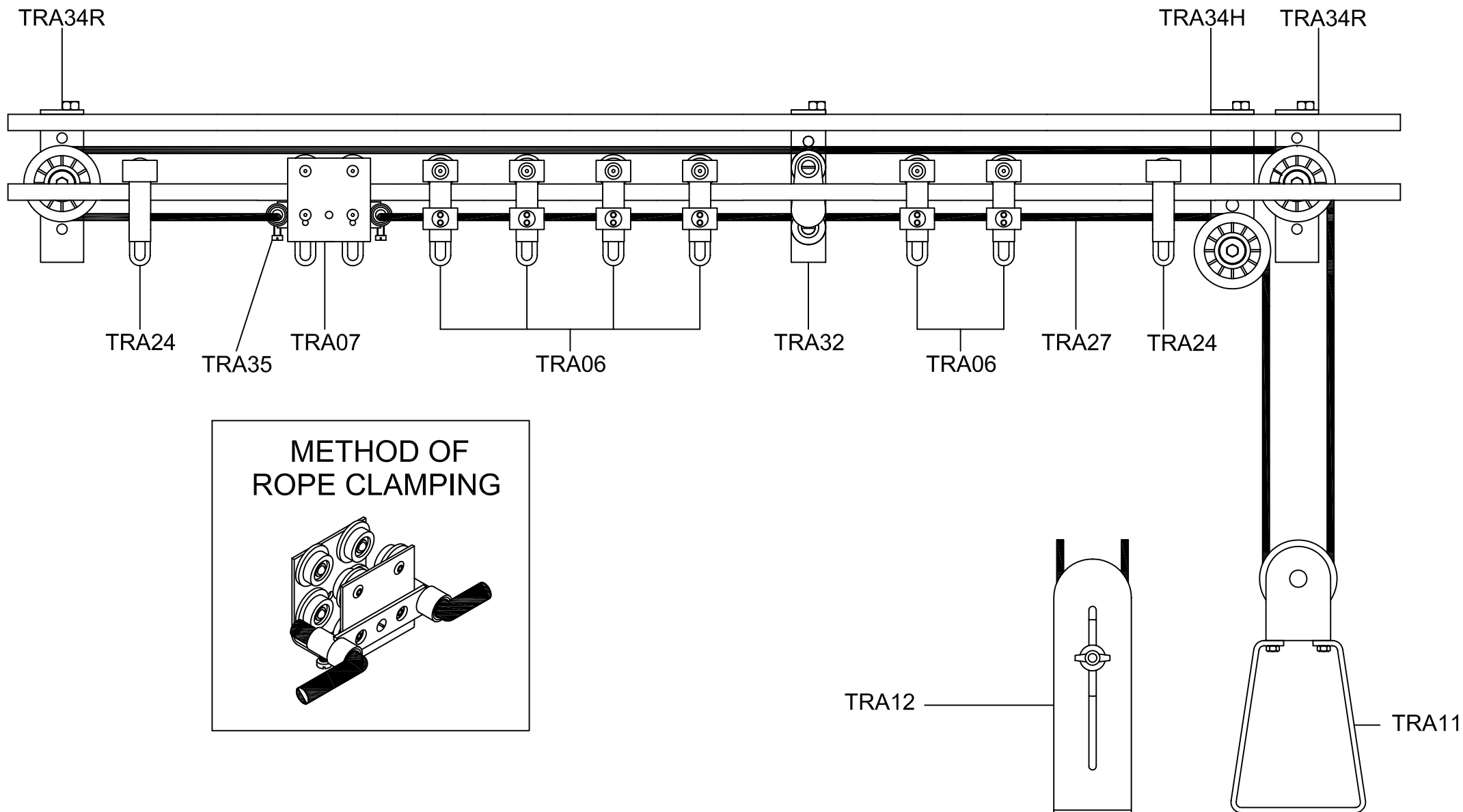
CORDING DIAGRAM 10 SIDE CORDED WIPE FOR CURTAINS VIEWED FROM SIDE
