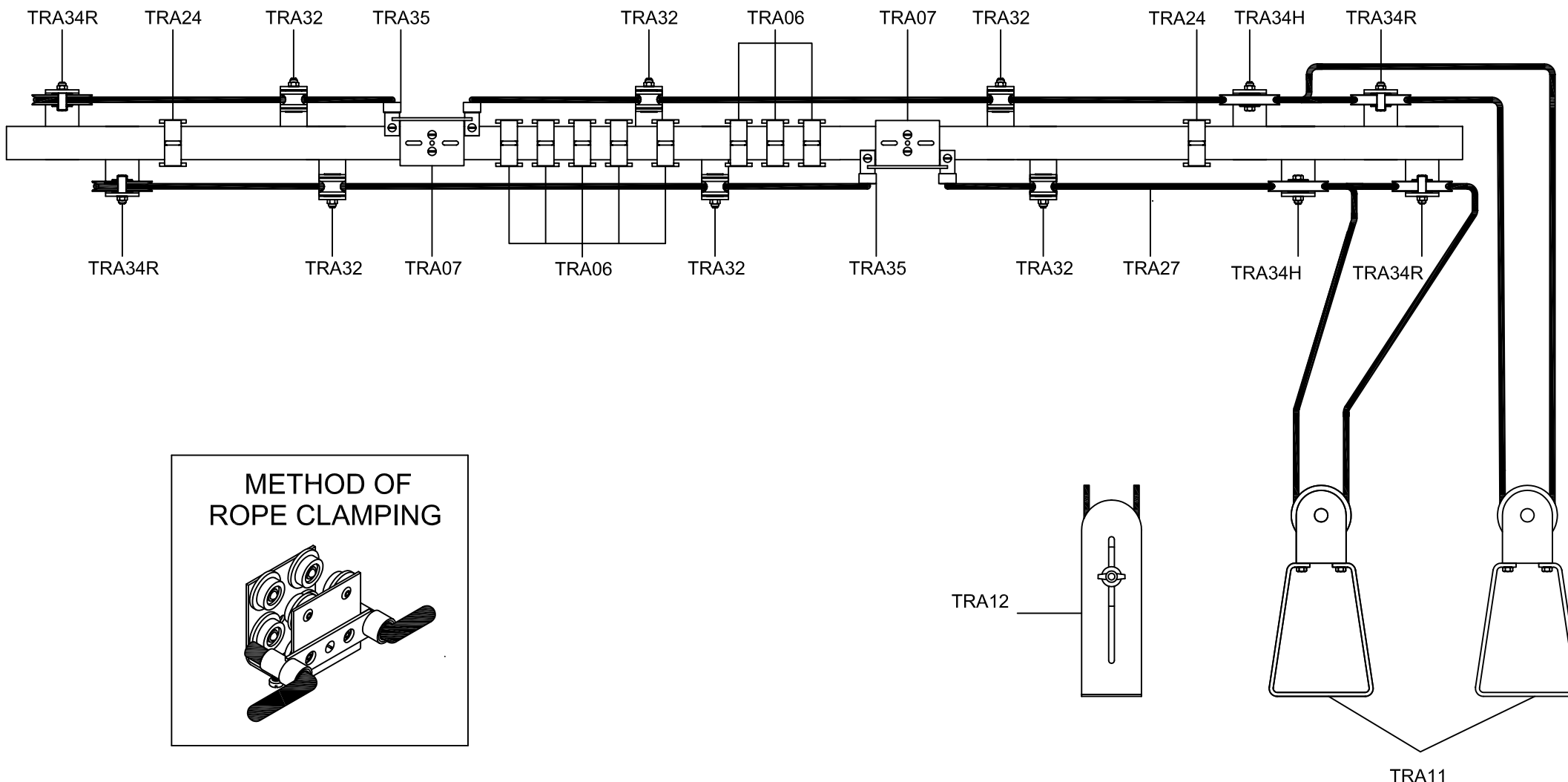
CORDING DIAGRAM 14 SIDE CORDING WITH INDEPENDENT MASTER RUNNERS VIEWED FROM UNDERSIDE
