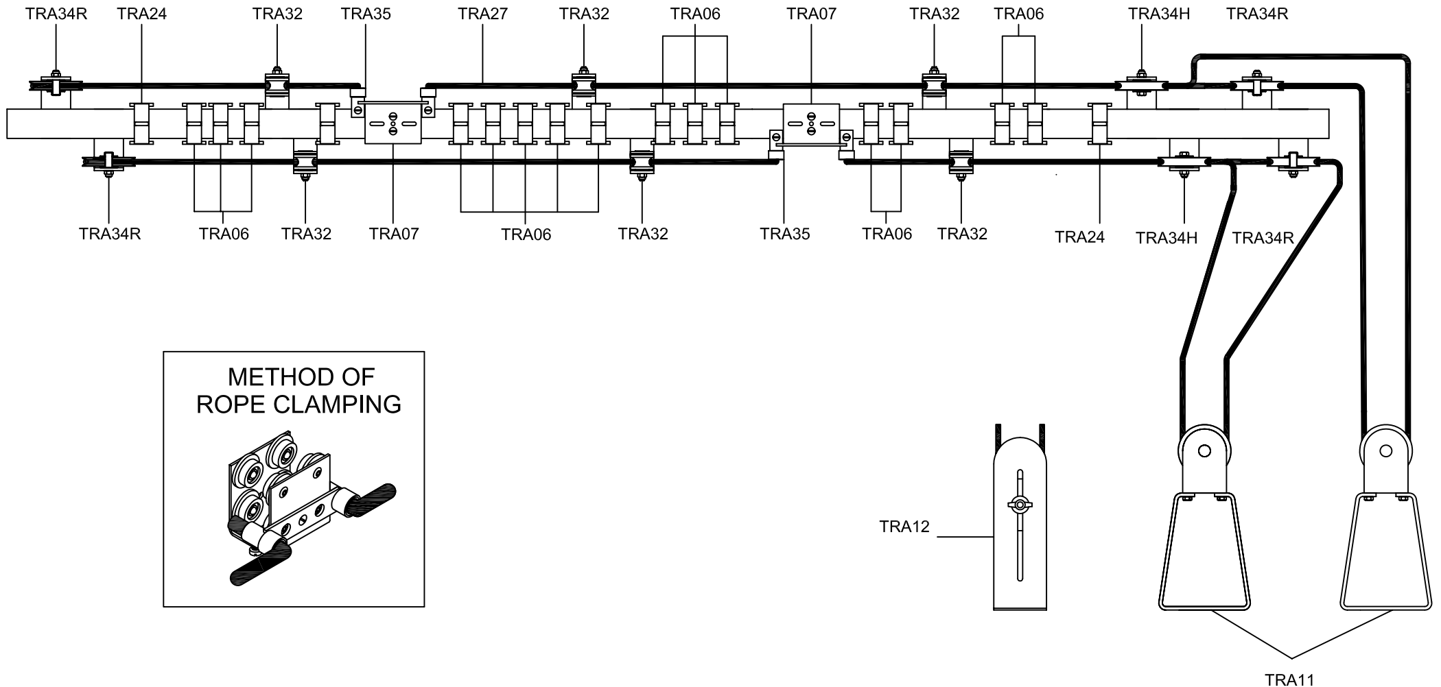
CORDING DIAGRAM 15 SIDE CORDING WITH INDEPENDENT MASTER RUNNERS FOR MULTIPLE CURTAINS VIEWED FROM UNDERSIDE
