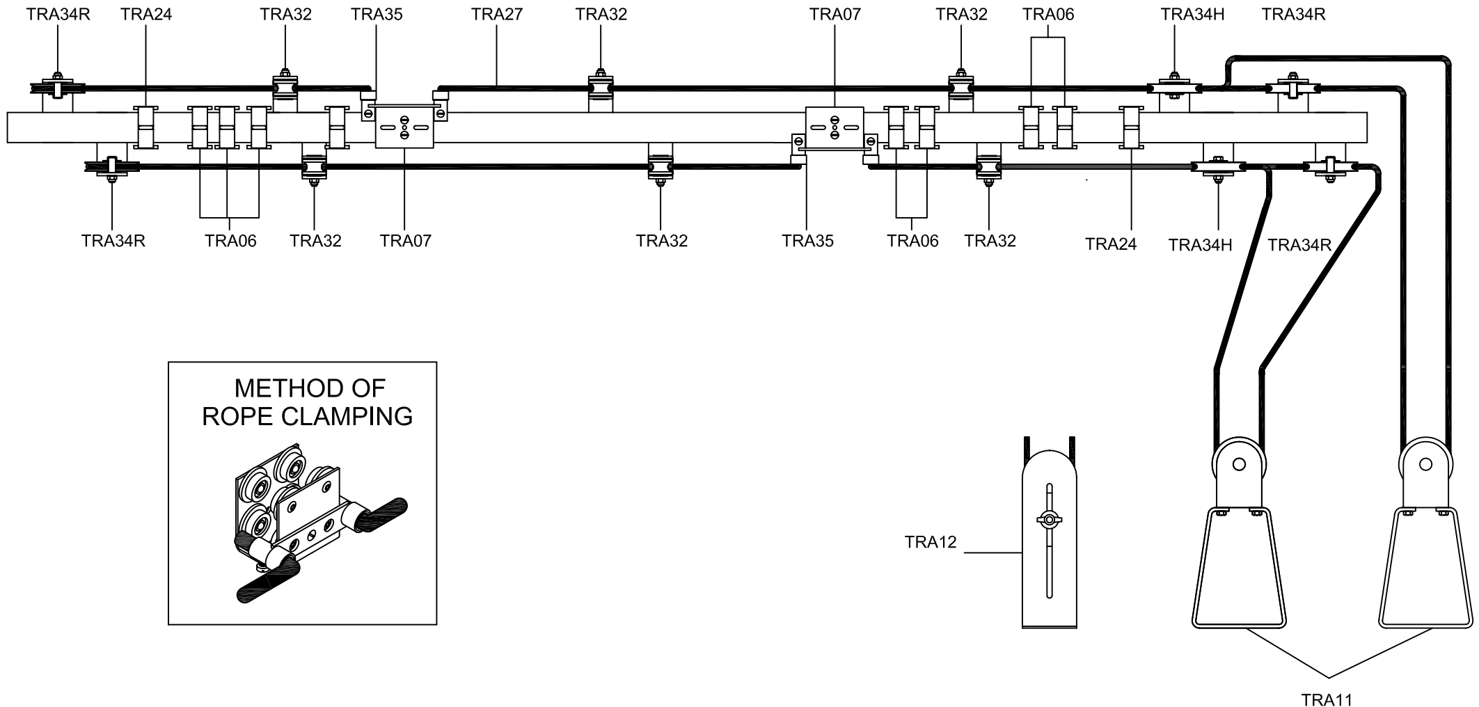
CORDING DIAGRAM 17 SIDE CORDING WITH INDEPENDENT MASTER RUNNERS FOR MULTIPLE CURTAINS VIEWED FROM UNDERSIDE
